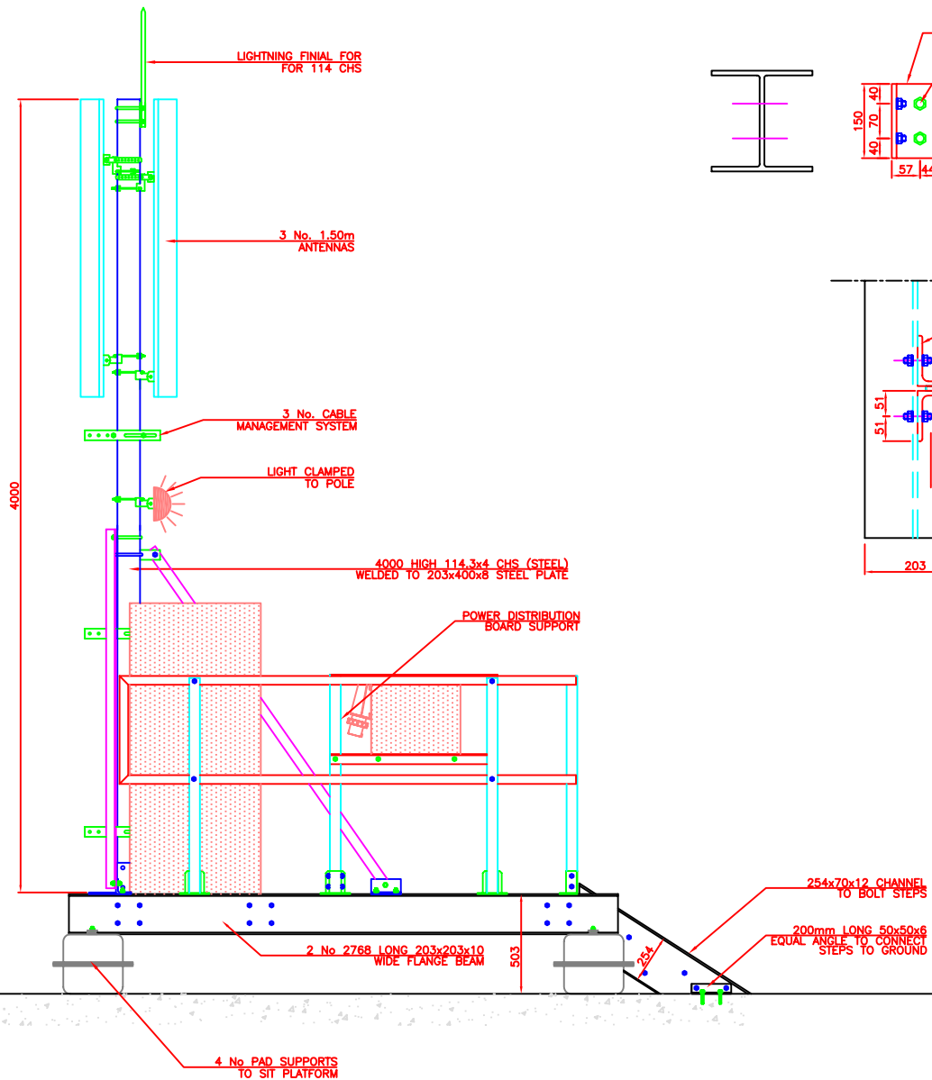
ELEVATION - A SCALE 1:25
